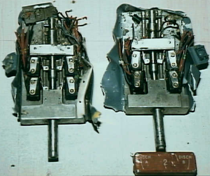
Systems 9 - Photo 2. Disassembly of the Engine Fire Handles
