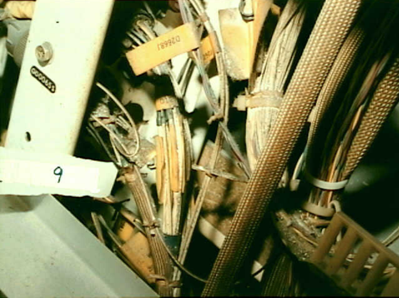
Systems 9 - Photo 18. Airplane 9. B-747 avionics rack wiring between stanchions and beneath drip shield. Metal shavings and lint coat the area. Raceway clamp is missing retainer at right.
