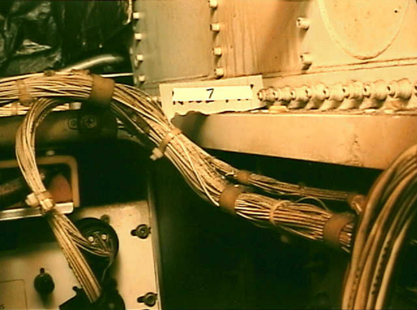
Systems 9 - Photo 12. Airplane 7. B-747 Drill shavings on wire bundles immediately beneath floor structure repair shown in photo 11. Fluid stain visible on structure.
