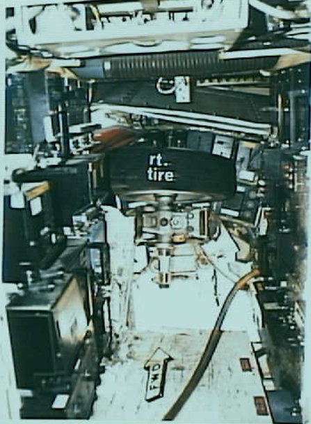
Systems 9 - Photo 11. View of E/E from the forward baggage compartment (looking forward). Note the nose gear folded back into the compartment clocked 90 degrees to the right. The left nose gear tire has been removed to gain access.
