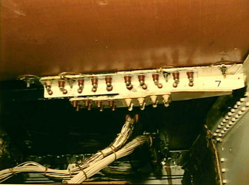
Systems 9 - Photo 11. Airplane 7. B-747 Floor structure repair in electrical equipment center, aft of station 400 (left side). Grouped open splices also visible in bundle.
