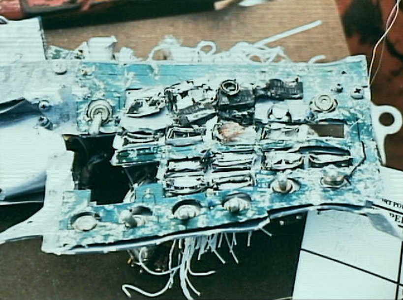
Systems 9 - Photo 1. Upper Portion of Ice and Rain Protection Panel
