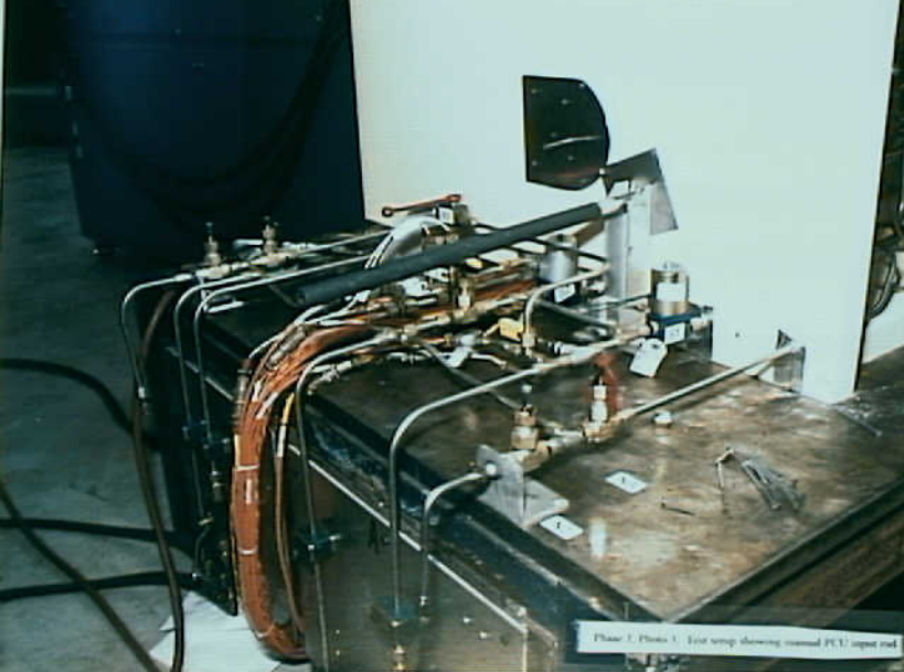
Systems 9 - Phase 2 - Photo 3. Test setup showing manual PCU input rod
