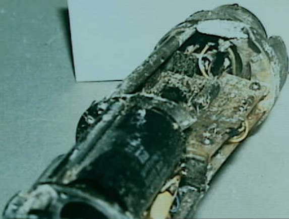
Systems 9 - Fuel Quantity Indicators - Photo 15. CWT indicator interior components and interior of connector, as photographed at NASA in August 1996.
