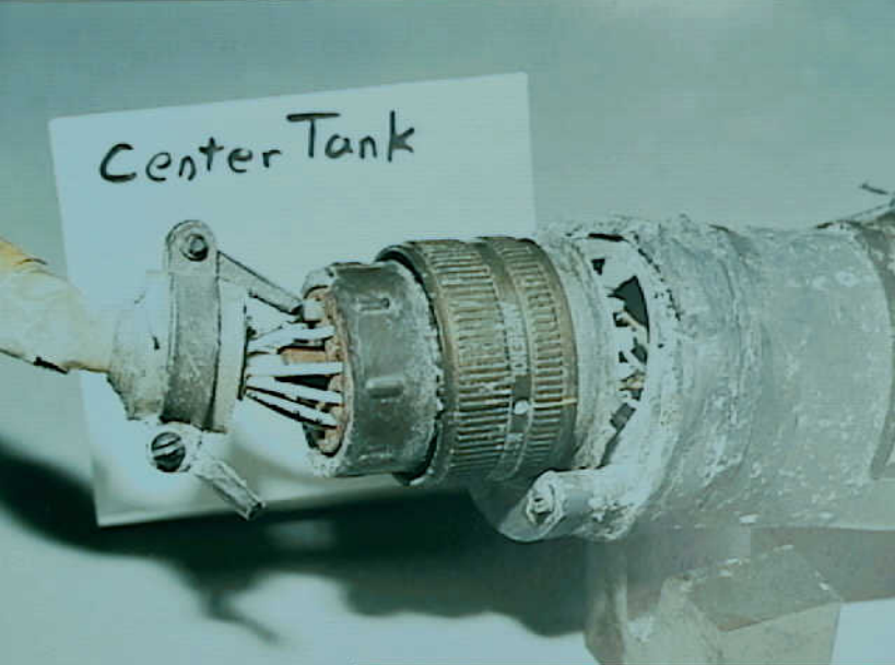
Systems 9 - Fuel Quantity Indicators - Photo 14. CWT connector and attached aircraft wire bundle (harness).
