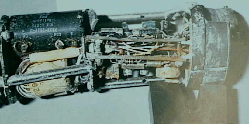
Systems 9 - Fuel Quantity Indicators - Photo 13. CWT indicator interior components.
