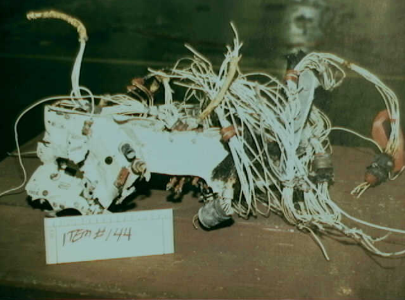
Systems 9 - Fuel Quantity Indication System - Photo 7. Wreckage of pressure refueling panel from left wing. (No negative available)
