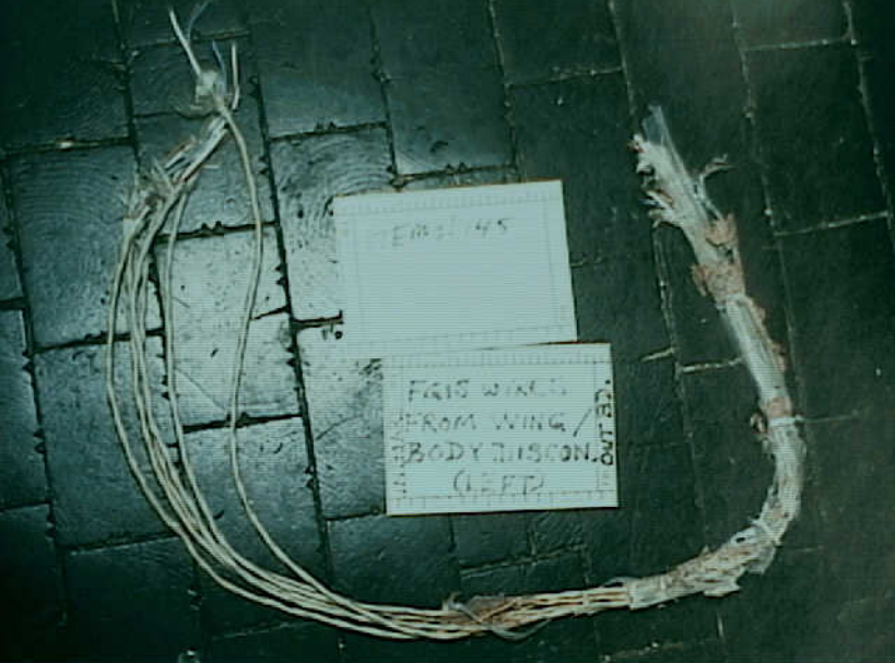
Systems 9 - Fuel Quantity Indication System - Photo 6. FQIS bundles from left wing/fuselage pressure seals. (No negative available)
