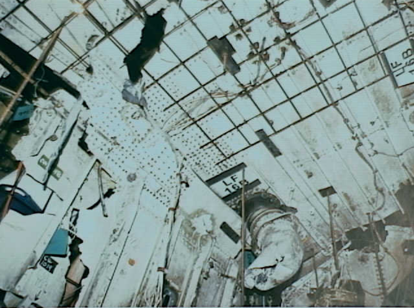
Systems 9 - Fuel Quantity Indication System - Photo 5. Left fuselage landing gear well, with location of DM127 connector on bottom edge, structural repair in midst of wire path, and pressure seals. (No negative available)
