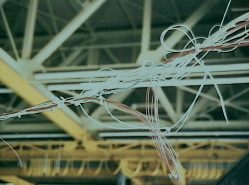
Systems 9 - Fuel Quantity Indication System - Photo 46. W480 (& other) bundles from upper deck at about station 420-480.
