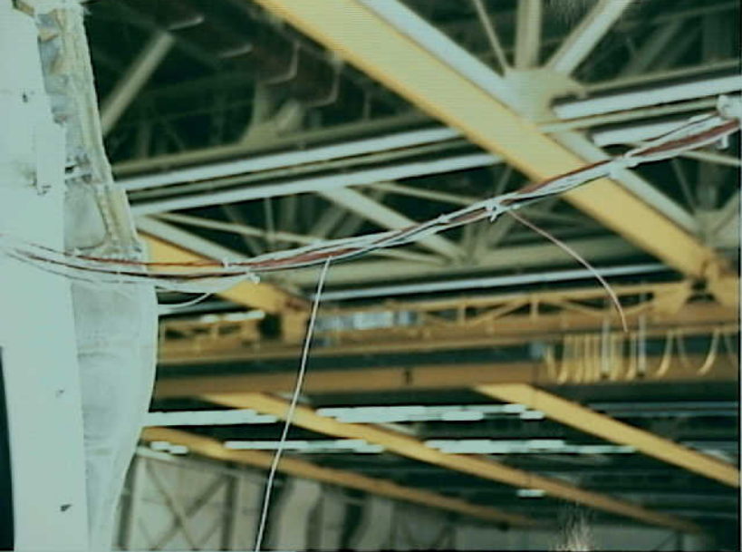
Systems 9 - Fuel Quantity Indication System - Photo 45. W480 (& other) bundles from upper deck at about station 480-520.
