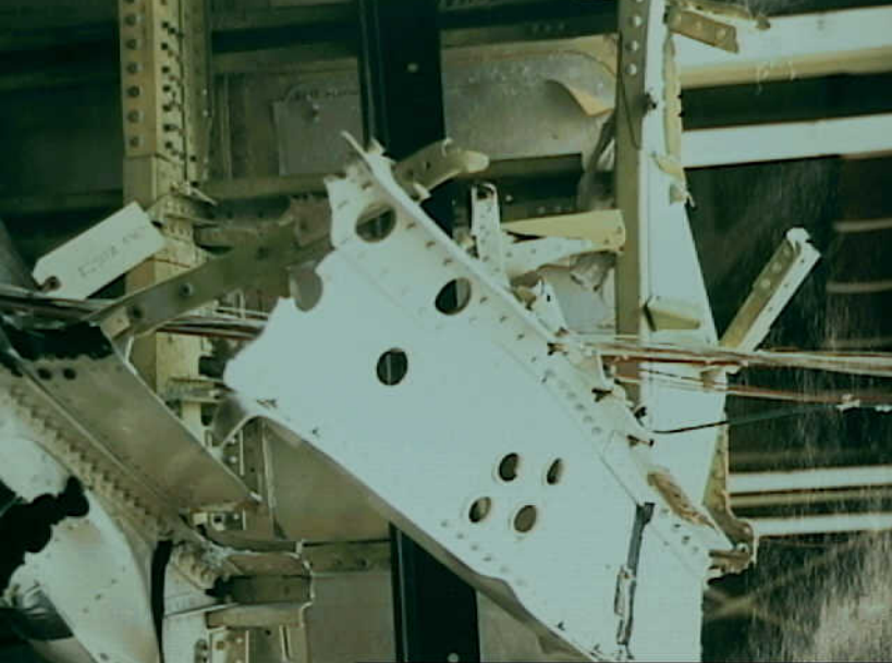
Systems 9 - Fuel Quantity Indication System - Photo 44. W480 (& other) bundles from upper deck at about station 500-540.
