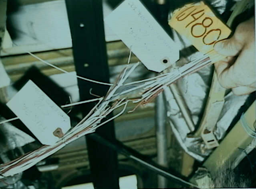
Systems 9 - Fuel Quantity Indication System - Photo 42. Detail of separation in W480 (& other) bundles from upper deck at about station 570.
