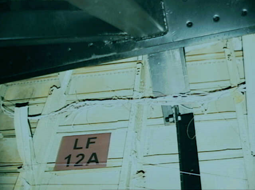
Systems 9 - Fuel Quantity Indication System - Photo 39. W480 (& other) bundles from upper deck at about station 850-920. (No negative)
