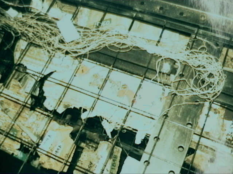
Systems 9 - Fuel Quantity Indication System - Photo 35. W480 (& other) bundles in reconstruction above tank, to about station 1250. Pressure seals are visible above left main landing gear well, as viewed downward from cabin.
