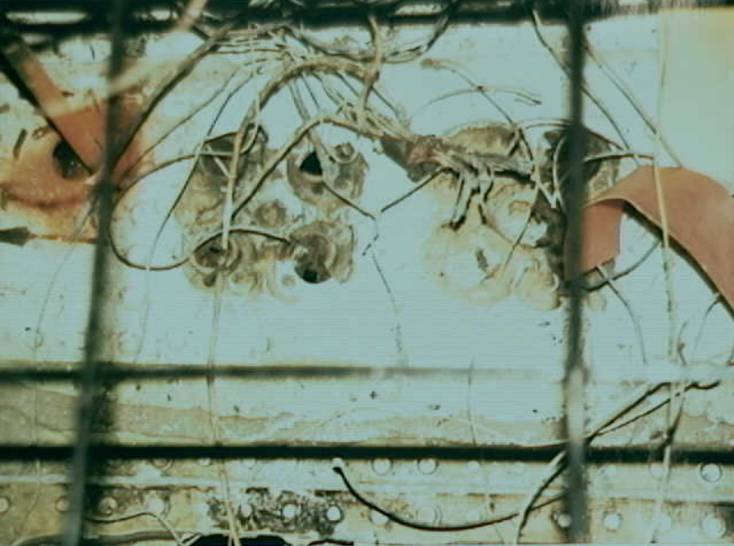
Systems 9 - Fuel Quantity Indication System - Photo 34. W480 (& other) bundle pressure seals above left main landing gear well, as viewed downward from cabin the floor removed.
