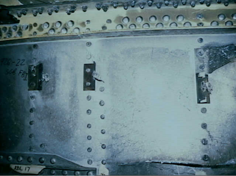
Systems 9 - Fuel Quantity Indication System - Photo 3. Attachment points of FQIS wires in CWT on spanwise beam 2. The T347 terminal strip attachment point is at right.
