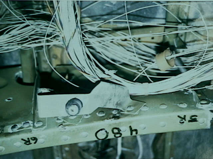
Systems 9 - Fuel Quantity Indication System - Photo 27. Darkened area on station 480 frame that is not visible on W985 wires from area.
