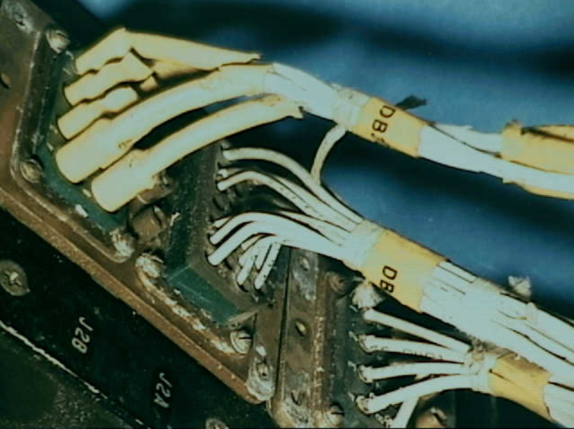
Systems 9 - Fuel Quantity Indication System - Photo 22. Wiring attachments at rear of VSO unit. Visible are the exposed conductors in the connector with fewest wires. (No negative available)
