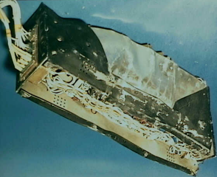
Systems 9 - Fuel Quantity Indication System - Photo 21. Bottom and back of VSO, showing external wiring (cut from E3-1 avionics shelf) and wiring internal to the unit. (No negative available)
