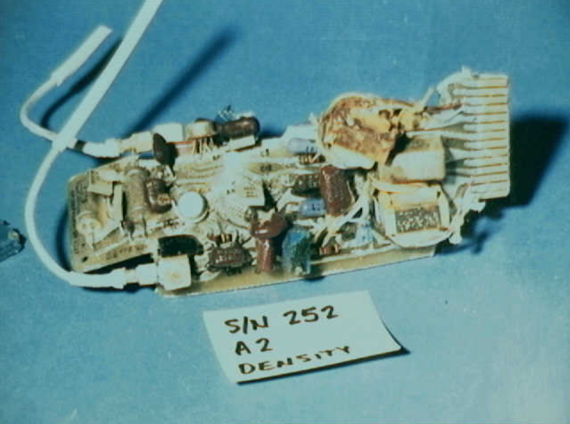
Systems 9 - Fuel Quantity Indication System - Photo 20. Typical circuit card from within the VSO. Edge with connector traces was downward in the installed position. (No negative available)
