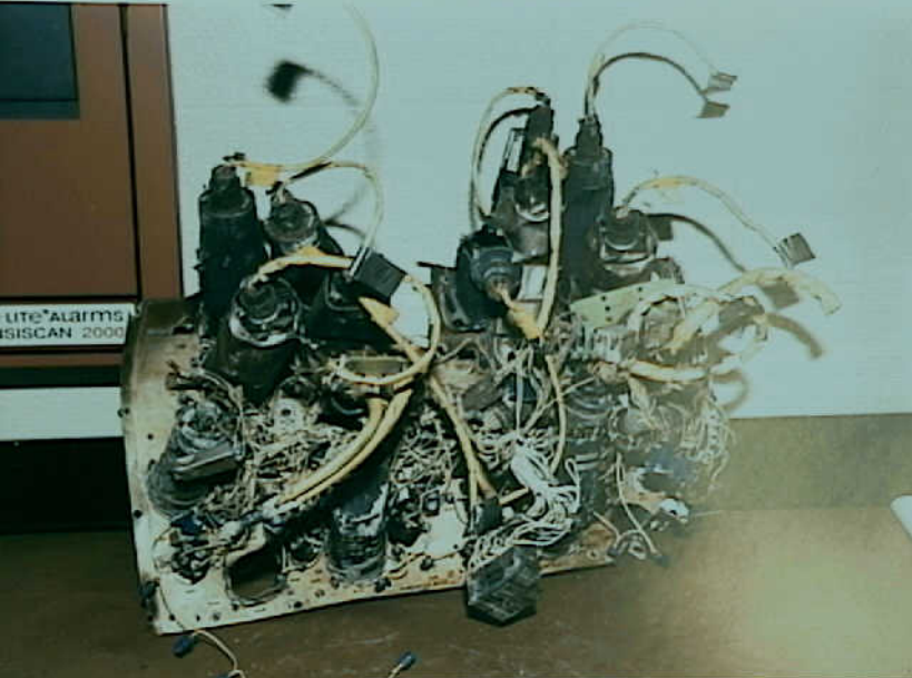
Systems 9 - Fuel Quantity Indication System - Photo 14. Back of flight engineer panel. (No negative available)
