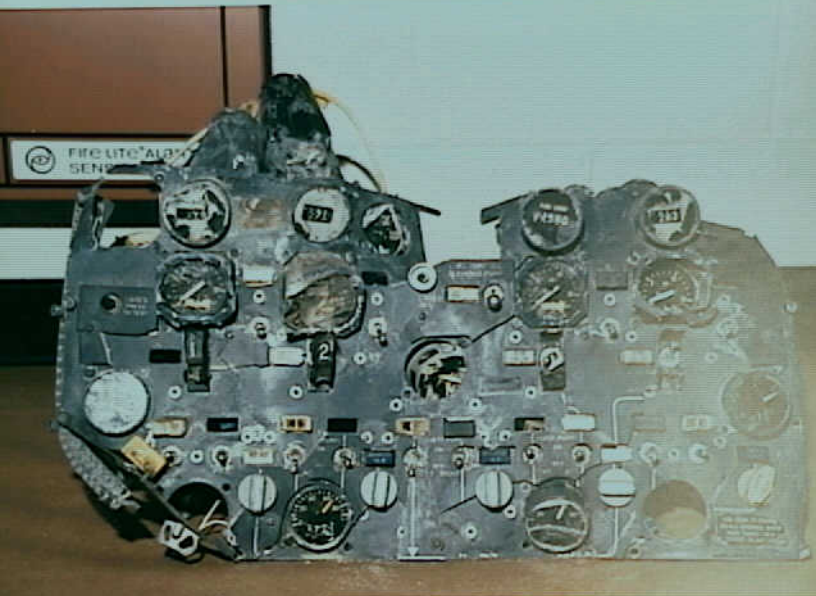
Systems 9 - Fuel Quantity Indication System - Photo 13. Face of flight engineer panel. (No negative available)
