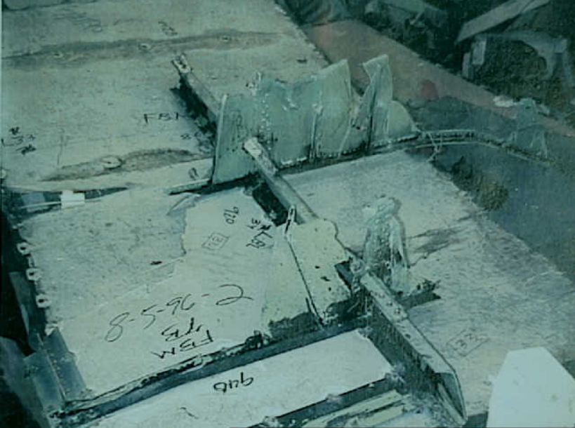
Systems 9 - Fuel Quantity Indication System - Photo 10. Structure repairs from bottom of main deck cabin floor. Large green item is back side of STA 920 floor beam and visible are black sealant and red fasteners. The part oriented from upper left to lower
