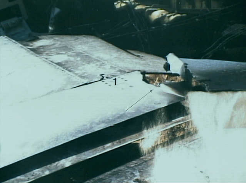
Systems 9 - Exhibit No. 9B - Photo 8. View (looking from left side) of spoiler control handle. Note only half of red ARM indicator (arrow) is visible.
