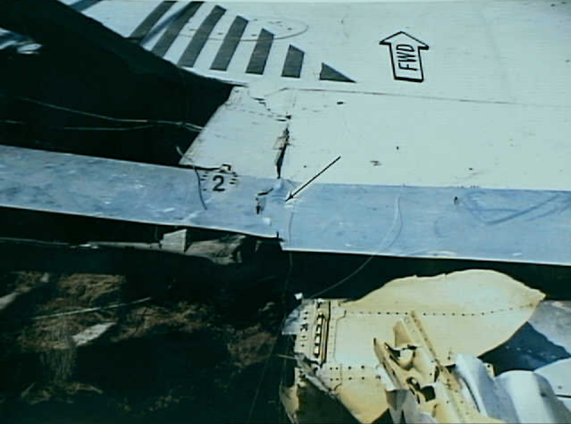
Systems 9 - Exhibit No. 9B - Photo 5. View (looking forward) of right inboard ground spoiler panel. Note the fracture (arrow) just outboard of actuator hinge (2).
