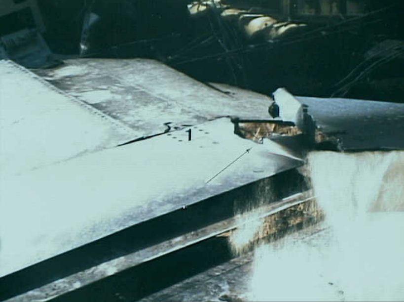
Systems 9 - Exhibit No. 9B - Photo 3. View (looking forward) of left inboard ground spoiler panel. Note the fracture (arrow) just inboard of actuator hinge (1) and extensive soot damage.
