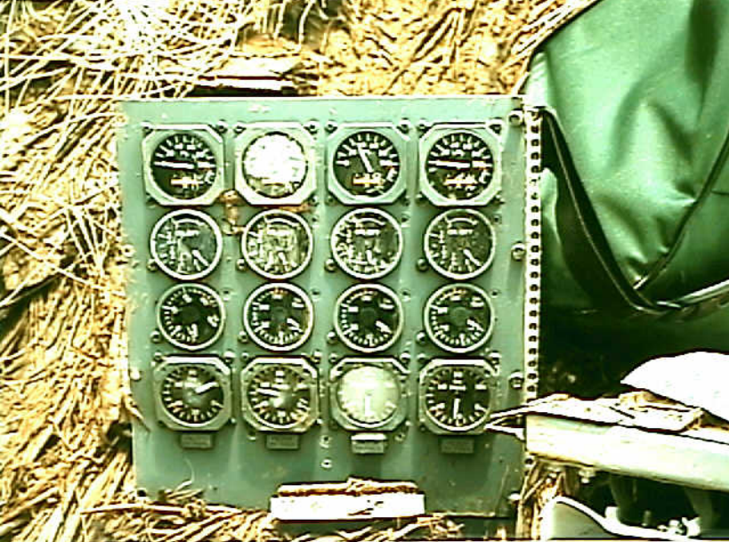
Systems 9 - Exhibit No. 9B - Photo 19. Flight Engineer's Engine Instrument Panel
