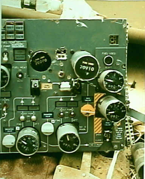
Systems 9 - Exhibit No. 9B - Photo 18. Flight Engineer's Fuel Control Panel
