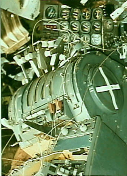
Systems 9 - Exhibit No. 9B - Photo 17. Throttle
