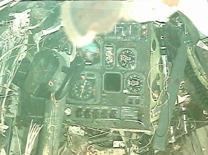
Systems 9 - Exhibit No. 9B - Photo 13. Captain's Instrument Panel
