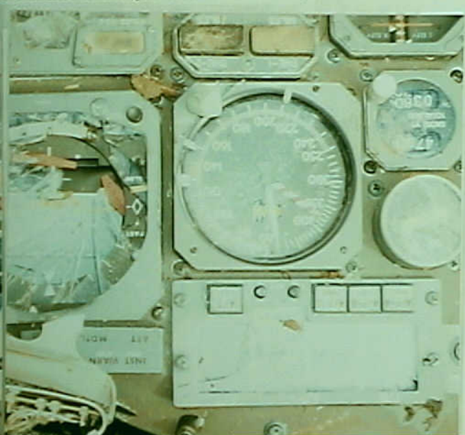
Systems 9 - Exhibit No. 9B - Photo 11. Close-up of First Officer's Instrument Panel
