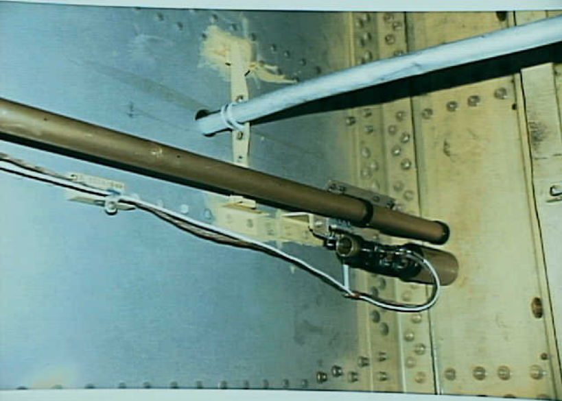
Systems 9 - Exhibit No. 9E - Photo No. 9 - CWT Fuel probe mounted forward of mid-spar with compensator and scavenge pump tube. Dents in probe and tube are visible. ( N93105). ATA 28-41-01.
