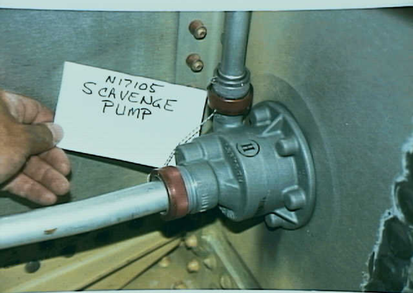
Systems 9 - Exhibit No. 9E - Photo No. 8 - Scavenge Pump. (N93105). ATA 28-15-00.
