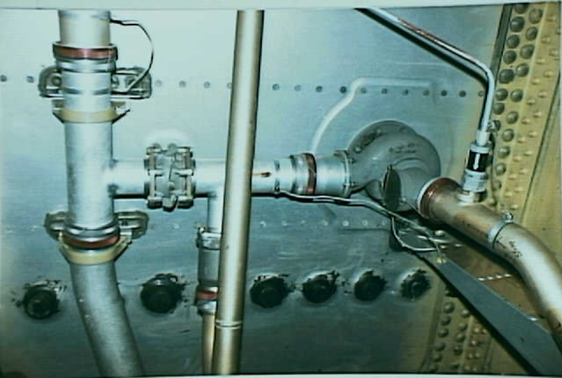
Systems 9 - Exhibit No. 9E - Photo No. 6 - Wiggins couplings (in red) connect fuel tubing in B-747 CWT (N93105). ATA 28-31-01.
