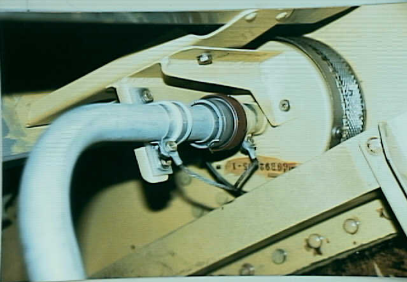
Systems 9 - Exhibit No. 9E - Photo No. 5 - Scavenge pick-up (N93105). ATA 28-15-00.
