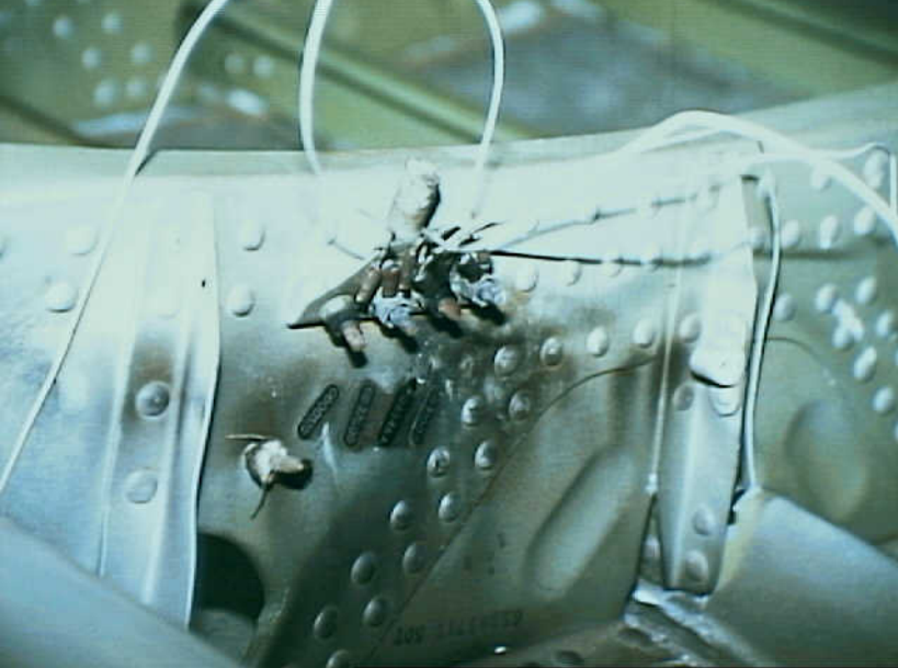
Systems 9 - Exhibit No. 9E - Photo No. 2 - Evidence of arcing along emergency light wire routing (to right of upper deck - N93119). ATA 24-50-00.
