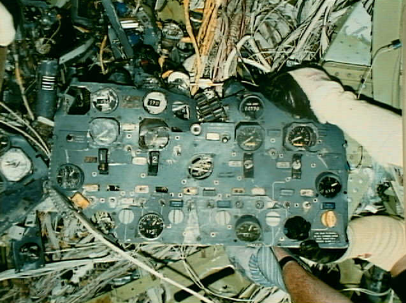
Systems 9 - Exhibit No. 9E - Photo No. 18 - Flight Engineer Fuel Panel (Cwt Indicator Behind)
