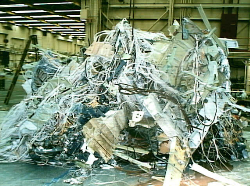
Systems 9 - Exhibit No. 9E - Photo No. 17. Flight Engineer Station & Cockpit Debris
