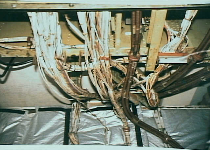
Systems 9 - Exhibit No. 9E - Photo No. 15 - FQIS wire routed with ships wiring which includes power wires. (N93105). ATA 28-41-09.
