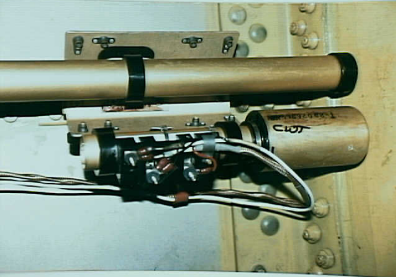
Systems 9 - Exhibit No. 9E - Photo No. 14 - CWT Fuel Compensator and lower portion of fuel quantity probe. (N93105). ATA 28-41-01.
