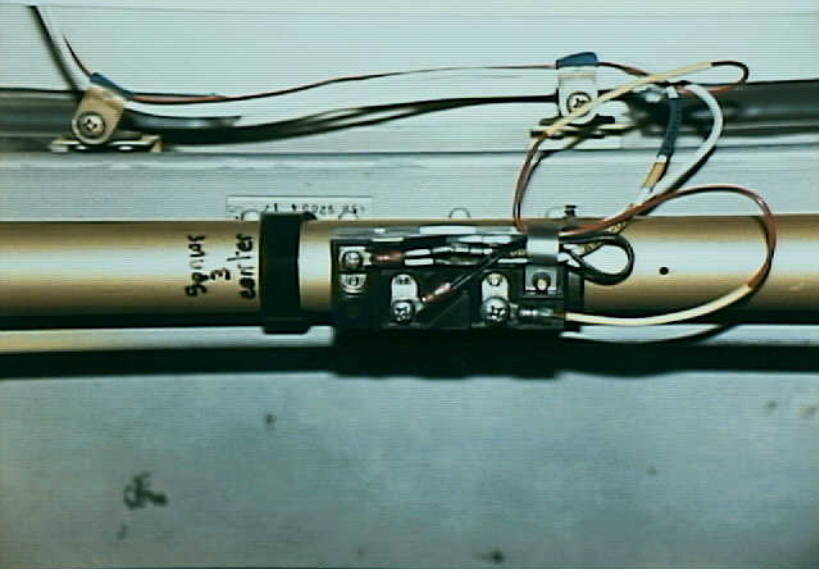
Systems 9 - Exhibit No. 9E - Photo No. 13 - CWT FQIS probe from forward center of CWT of N93105, showing red wire under clamp. ATA 28-41-01.
