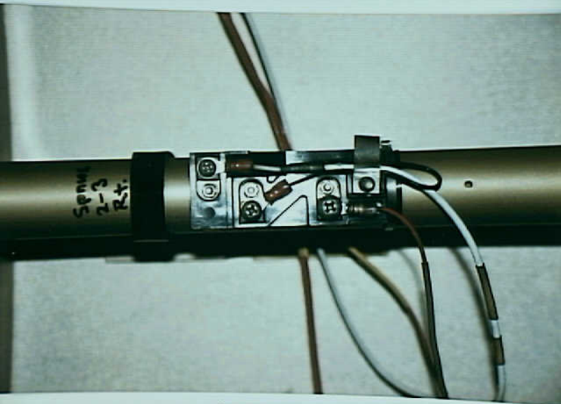
Systems 9 - Exhibit No. 9E - Photo No. 12 - CWT FQIS probe from forward right corner of CWT of N93105, showing red wire under clamp. ATA 28-41-01.
