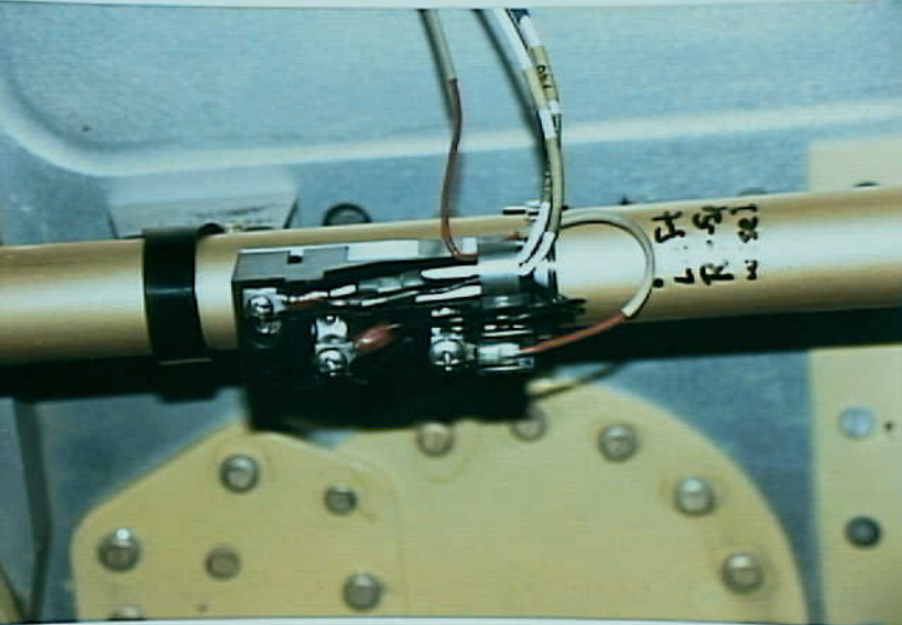
Systems 9 - Exhibit No. 9E - Photo No. 11 - CWT FQIS probe from left rear bay of N93105, showing red wire under clamp. ATA 28-41-01.
