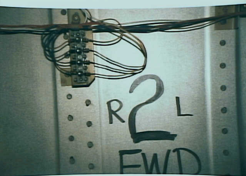
Systems 9 - Exhibit No. 9E - Photo No. 10 - CWT FQIS terminal block in N93105. Right wing FQIS wires routed to refuel panel in left wing are shown. ATA 28-40-00.
