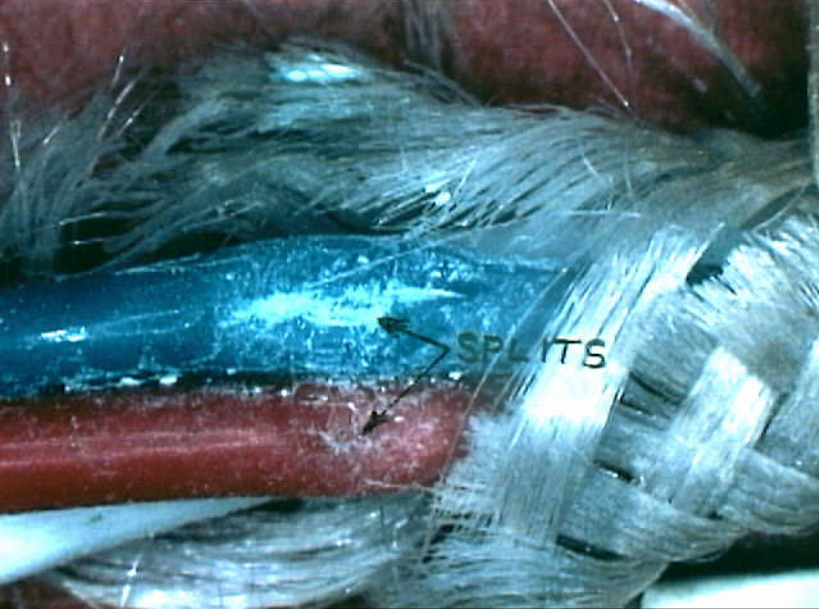
Systems 9 - Exhibit No. 9C - Photo 2 - Splits found in W480 Bundle from N93119 CWT FQIS. Source was external to CWT, in Routing to Cockpit.
